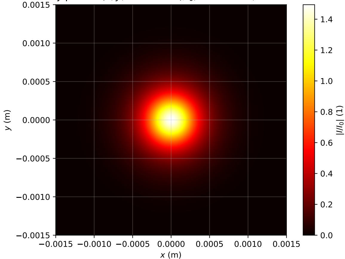
Intensity profile I(x, y, z = 0.955m)/I_0 , Pin=1.0Pcr, artificial time
